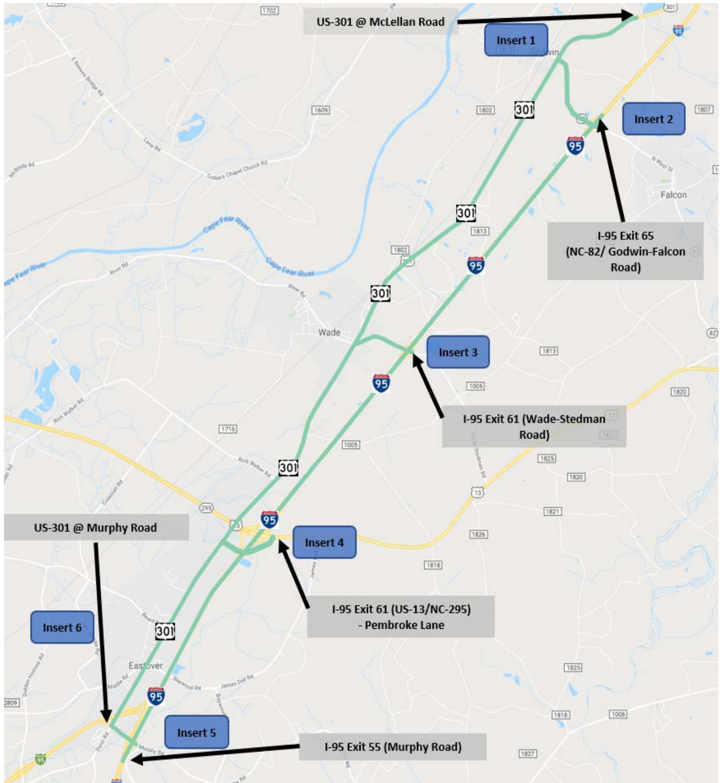
Figure 2: Heavy-Duty Zone 2 Coverage Area
